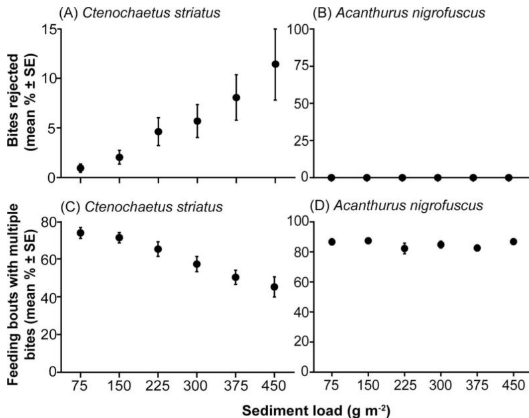
Fig 3. The behavioural response of two surgeonfishes to increasing sediment loads. The percentage of bites rejected (mean \pm SE) by (A) Ctenochaetus striatus , ( n = 24 ) and (B) Acanthurus nigrofuscus , ( n = 28 ) and the percentage of feeding bouts with multiple bites (mean \pm SE) by (C) C. striatus ( n = 24 ) and (D) A. nigrofuscus ( n = 28 ).
