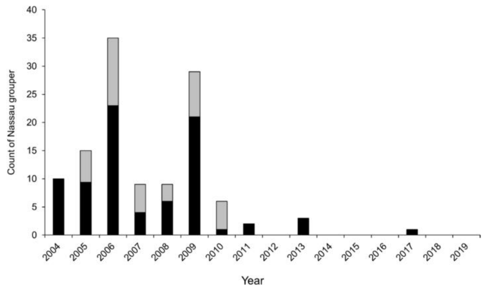
Fig. 11 Bar graph showing total number/year and proportional distribution of legal catch and undersized catch of Nassau grouper ( n=119 ) in fishery-dependent dataset from Glover's Reef Marine Reserve 2004–2019. Black portion = undersized catch (<50 cm). Grey portion = legal catch (50–74 cm). No mega spawner oversized (> 76 cm) individuals were recorded
