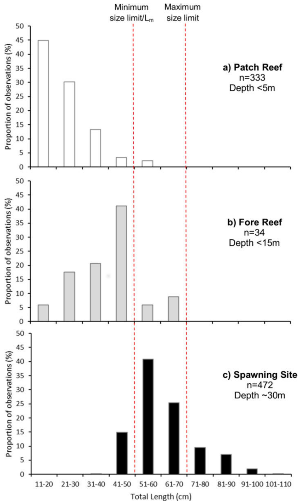
Fig. 8 Proportional distribution of length frequencies of Nassau groupers in patch reef survey data collected 2004–2022 ( n=333 ), fore reef survey data collected 2015–2023 ( n=34 ) and laser calliper data from Northeast Point FSA collected 2017–2023 ( n=472 ). Mean size of individuals is higher in ascending order from patch reefs ( 24.3 \pm 0.6 ) to fore reefs ( 42.4 \pm 2.5 ) to the spawning site ( 60.9 \pm 0.5 ). Shapiro–Wilk tests of normality returned p < 0.001 for patch reef length frequencies, p = 0.038 for fore reef, and p < 0.001 for FSA
