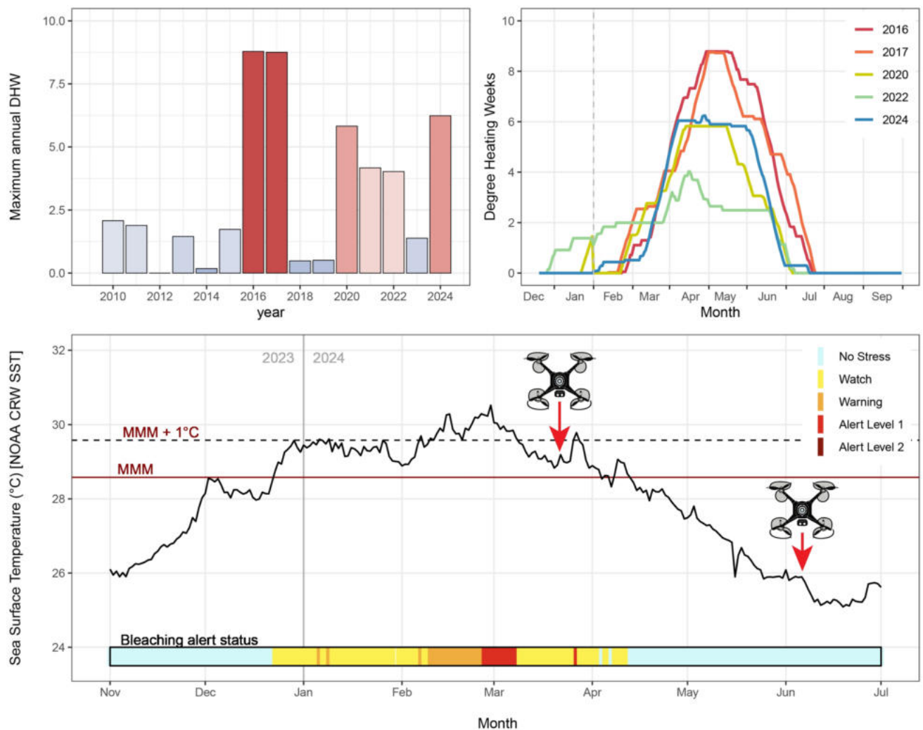
Fig. 5 Bleaching alert level inferred from sea surface temperature (SST), and degree-heating weeks (DHW) for Lizard Island, QLD, Australia in 2024 (bottom), and in previous years (top). Note the drones and arrows indicating when imagery was collected relative
