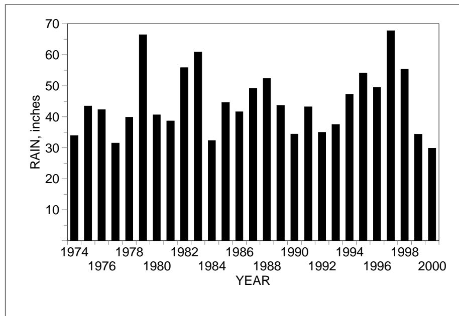
Figure 8. Rainfall at the Tampa International Airport measured by the National Oceanographic and Atmospheric Administration, National Climatic Data Center.
